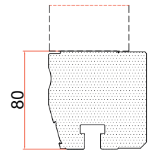
Wila American Type Hydraulic Punch Clamping
