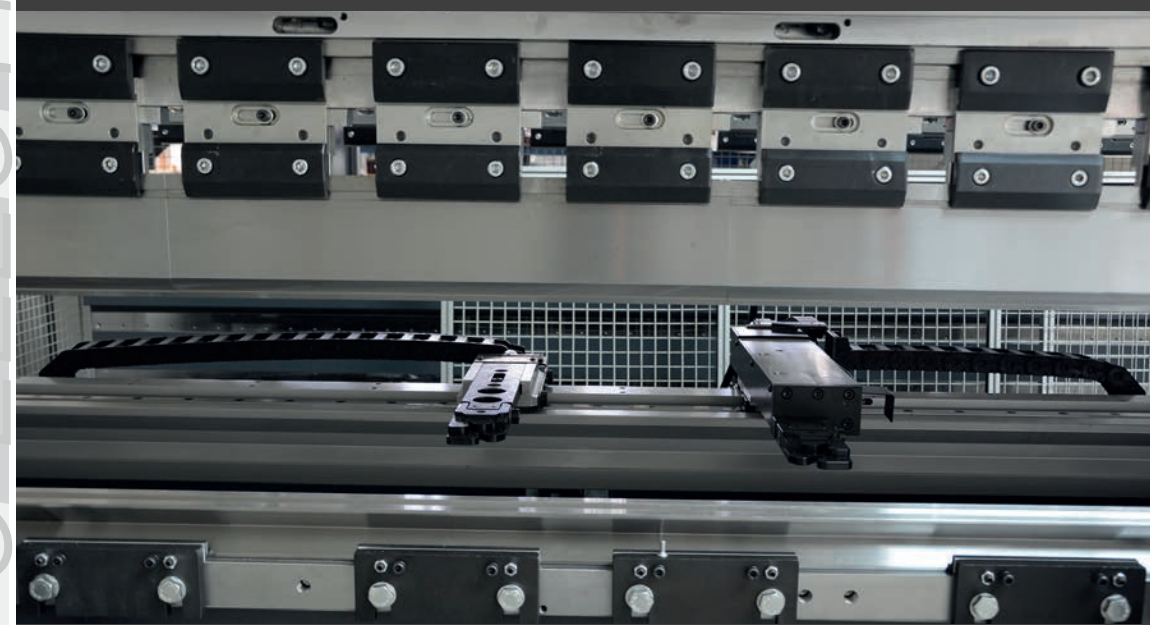
X - PRIME BACK GAUGE OPTION
