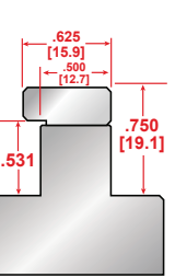
American Style Punch
